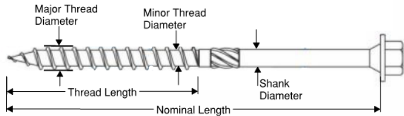
FIGURE 2. GL GRAY STRUCTURAL SCREW
