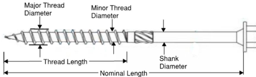
FIGURE 1. BL LOG, TIMBER & LANDSCAPING SCREW
