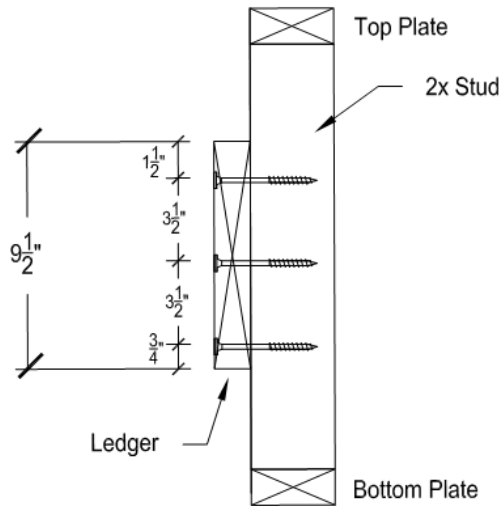
FIGURE 7. 2X10 LEDGER DIRECTLY ATTACHED TO STUD
