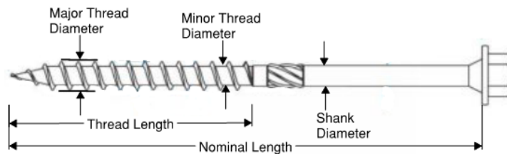
FIGURE 2. BL LOG, TIMBER & LANDSCAPING SCREW
