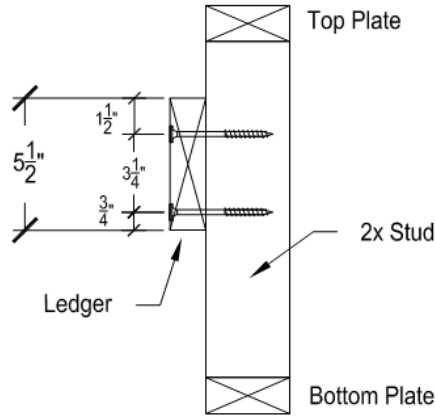
FIGURE 5. 2X6 LEDGER DIRECTLY ATTACHED TO STUD
