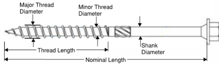
FIGURE 3. GL GRAY STRUCTURAL SCREW
