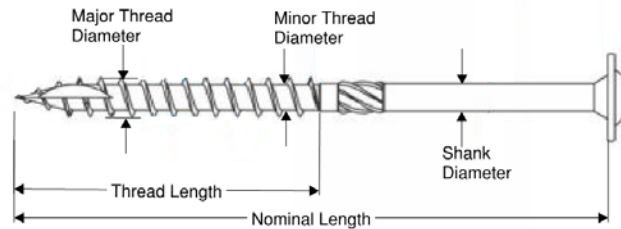
FIGURE 1. BIG TIMBER® CTX CONSTRUCTION LAG SCREW
